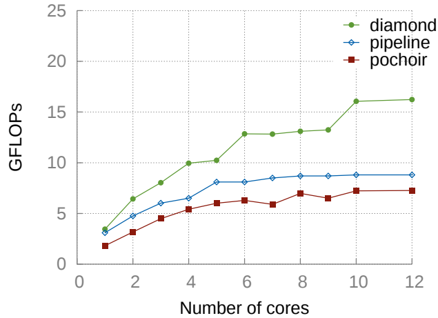
Figure 8.10: 3d-heat-periodic
