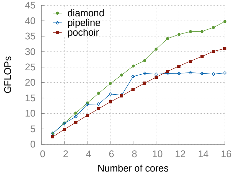
Figure 8.3: 2d-heat (AMD)
