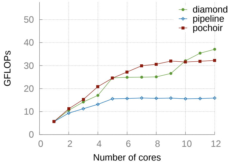
Figure 8.4: 3d-heat
