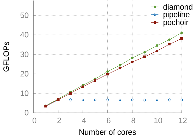
Figure 8.2: 1d-heat
