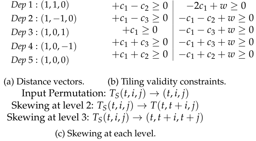
Figure 4.6: Skewing in heat-2d benchmark.
